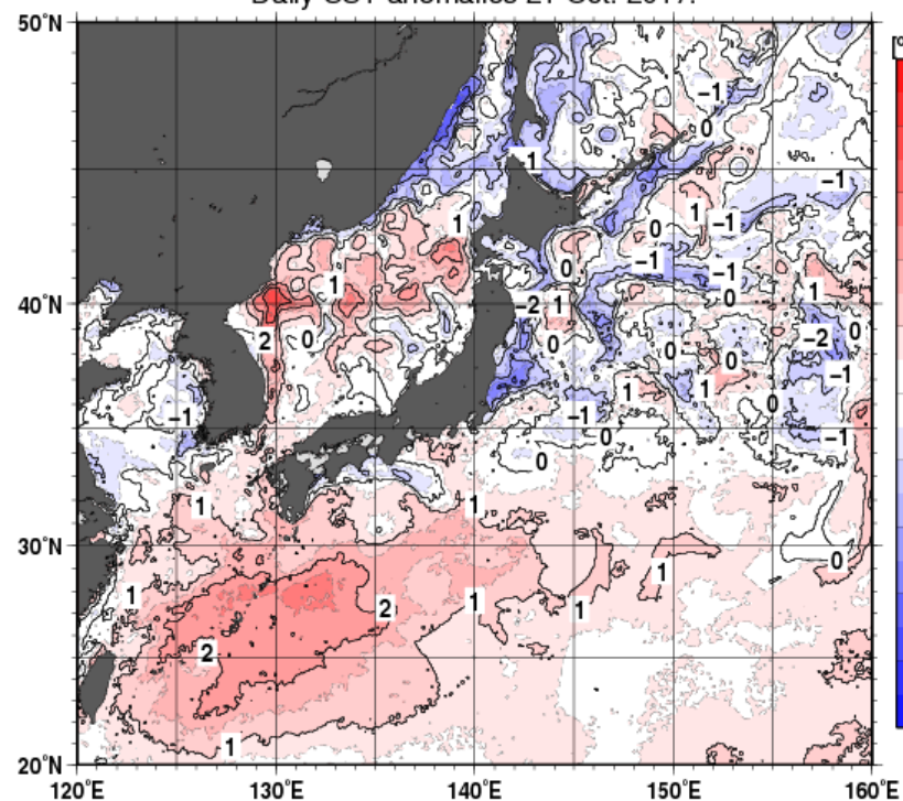
Daily SST anomalies 21 Oct. 2017.
