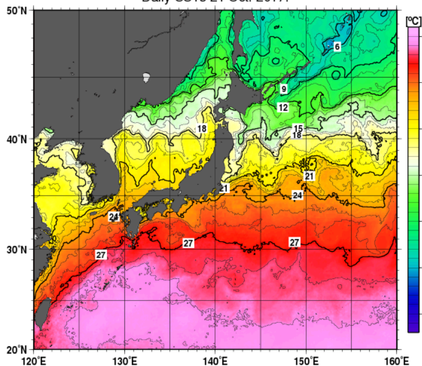
Daily SSTs 21 Oct. 2017.
